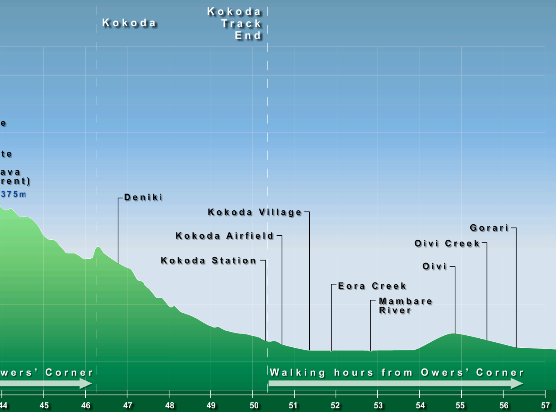
Topography of the Kokoda track
